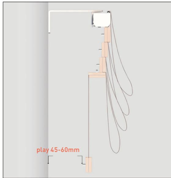
Fitted with extension bracket (added price option)
